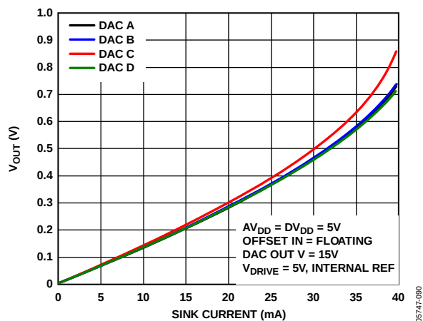
Figure 25. DAC Sinking Current at Input Code = x000, ( V_{OUT} = 0\text{ V} )
