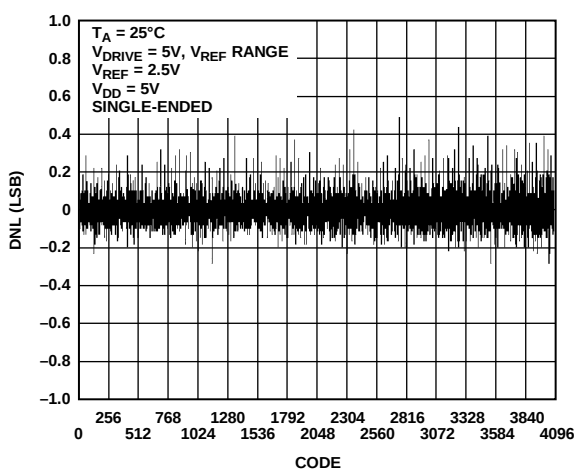
Figure 11. ADC DNL Single-Ended, V_{REF} Range
