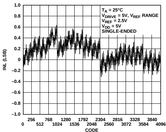
Figure 10. ADC INL Single-Ended, V_{REF} Range
