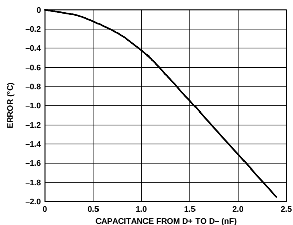
Figure 30. Temperature Error vs. Capacitor Between D+ and D-
