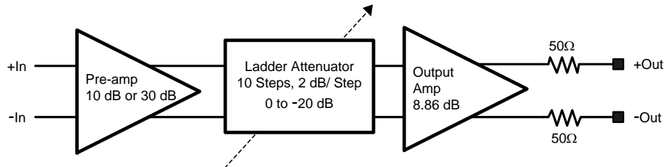
Figure 57. LMH6518 Signal Path Block Diagram
