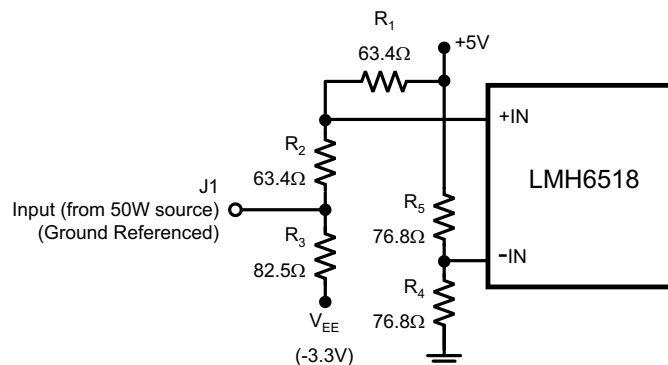
Figure 60. LMH6518 Driven by a Ground Referenced Source
