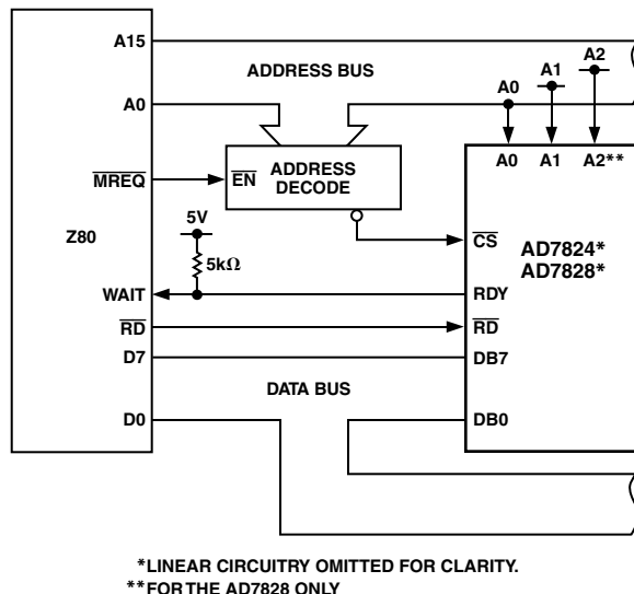
Figure 16. AD7824/AD7828-Z80 Interface
