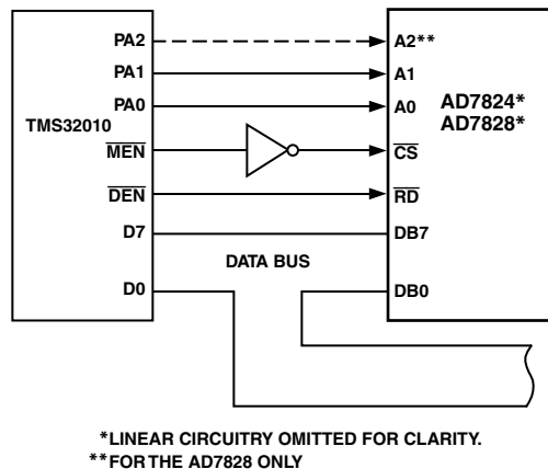
Figure 18. AD7824/AD7828–TMS32010 Interface
