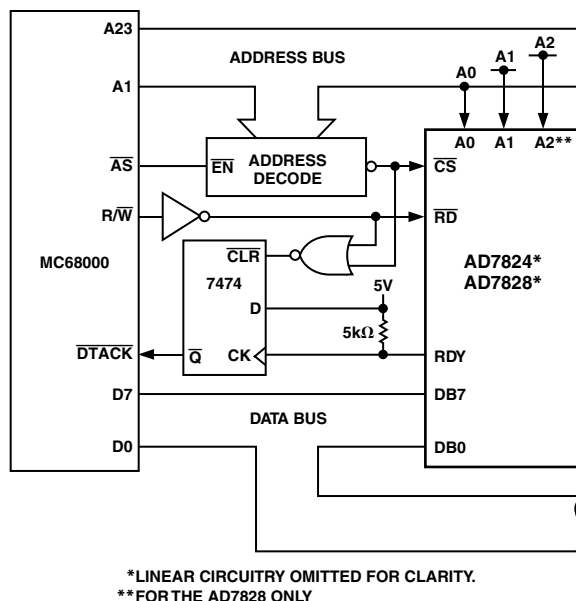
Figure 17. AD7824/AD7828–MC68000 Interface
