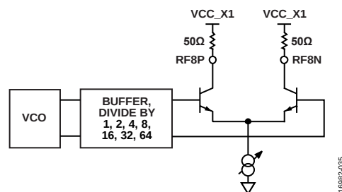
Figure 41. Output Stage
