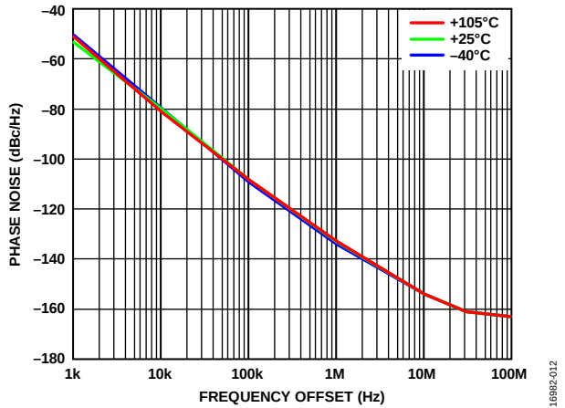
Figure 12. Open-Loop VCO Phase Noise over Temperature, 8.0 GHz, V_{CC\_VCO} = 5\text{ V}
