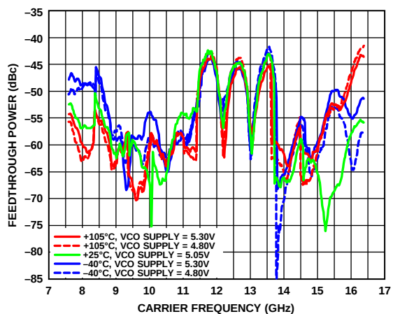
Figure 18. RF16P and RF16N VCO Feedthrough, De-Embedded Board and Cable Measurement, Combined Using Balun
