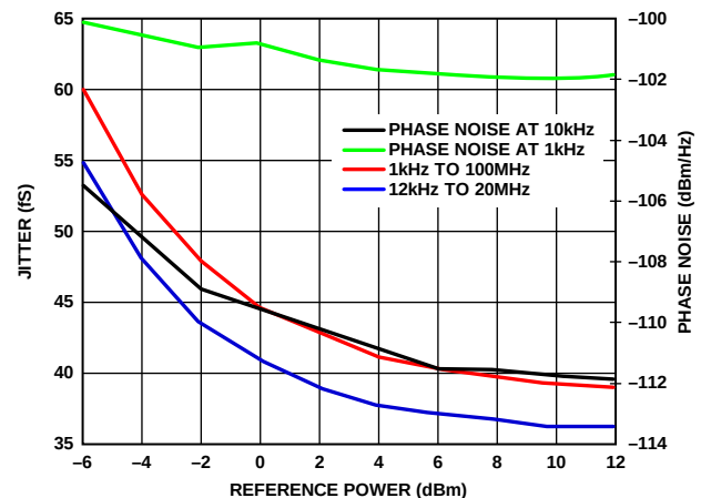
Figure 33. Jitter and Phase Noise, f_{PFD} = 250 \text{ MHz}
