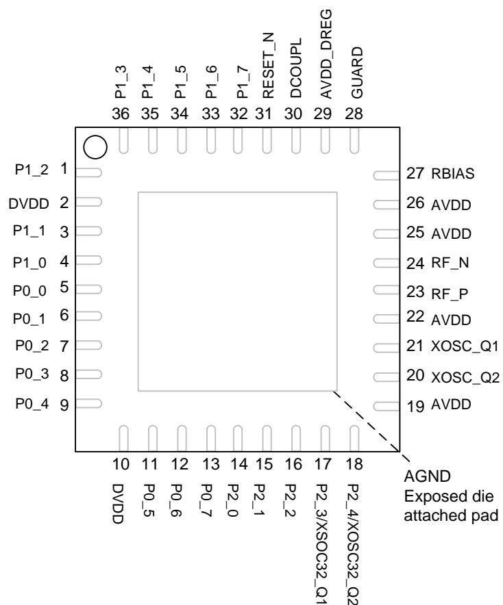
Note: The exposed die attach pad must be connected to a solid ground plane as this is the ground connection for the chip.
