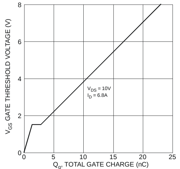
Figure 10 Gate Charge
