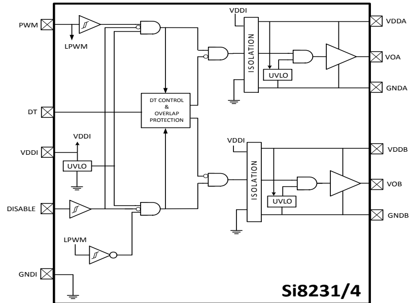
Figure 2.2. Si8231/4 Single-Input High-Side/Low-Side Isolated Drivers
