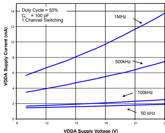
Figure 2.25. Supply Current vs. Supply Voltage
