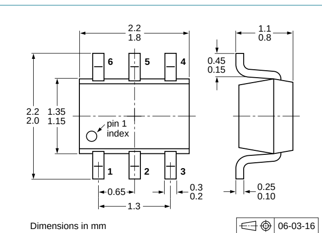
Fig 17. Package outline PUMD15 (SOT363)
