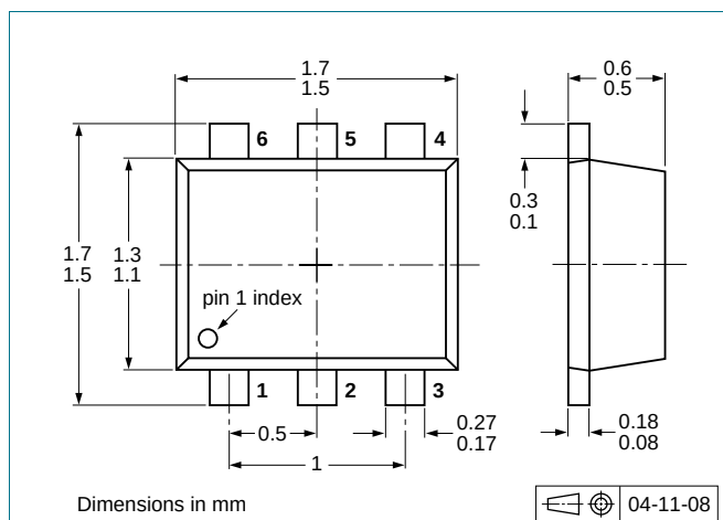
Fig 16. Package outline PEMD15 (SOT666)
