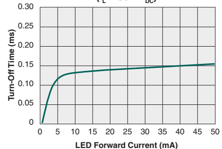
Typical Turn-Off Time vs. LED Forward Current ( I_L=130\text{mA}_{DC} )
