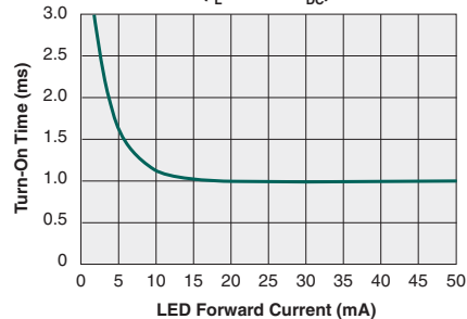
Typical Turn-On Time vs. LED Forward Current ( I_L=130\text{mA}_{DC} )
