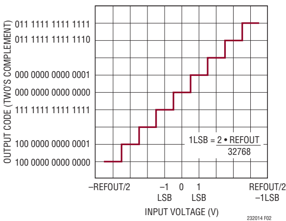
Figure 2. LTC2320-14 Transfer Function
