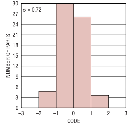
DC Histogram
