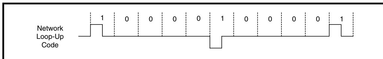
FIGURE 34. NETWORK LOOP UP CODE GENERATION
