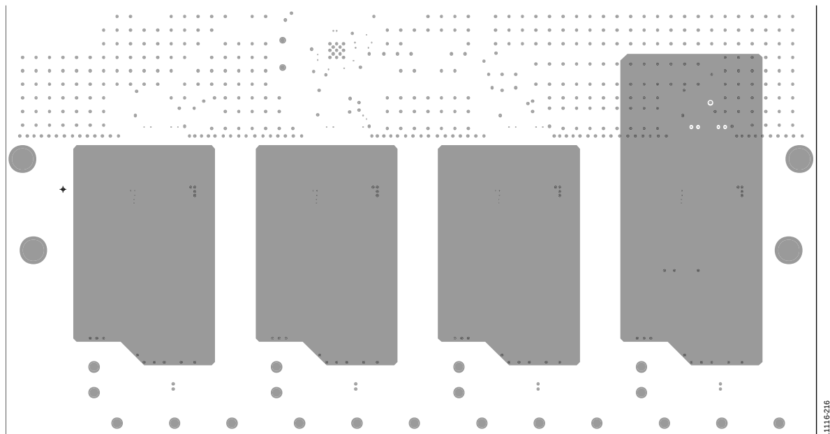
Figure 121. ADE7978, ADE7933, and ADE7923 Circuit Board, Layer 2
