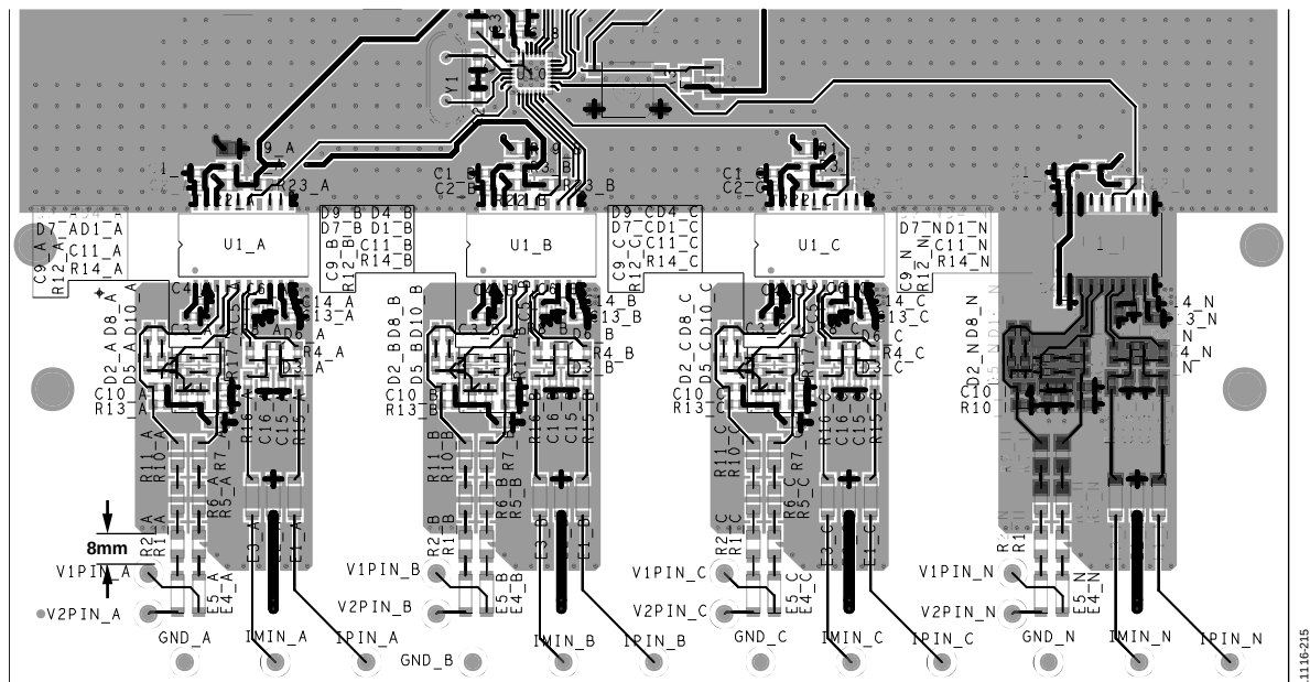
Figure 120. ADE7978, ADE7933, and ADE7923 Circuit Board, Layer 1
