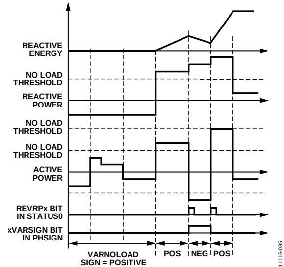
Figure 99. Reactive Power Sign Adjusted Mode
