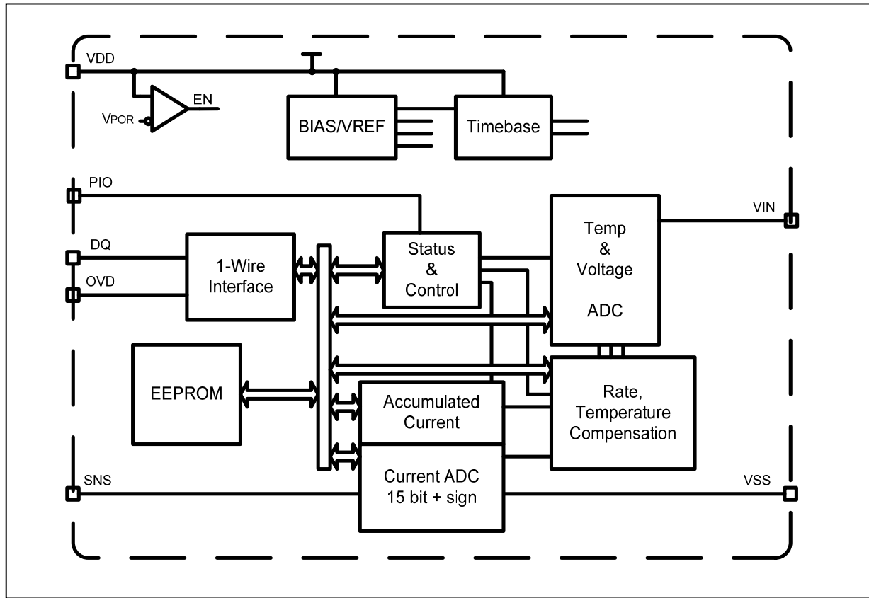
Figure 1. Block Diagram
