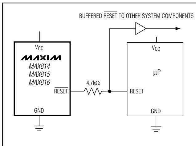
Figure 14. Interfacing to µPs with Bidirectional Reset I/O
