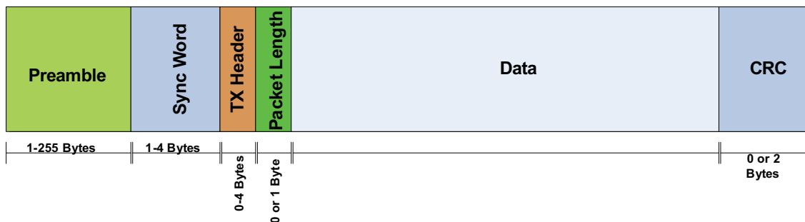
Figure 18. Packet Structure
