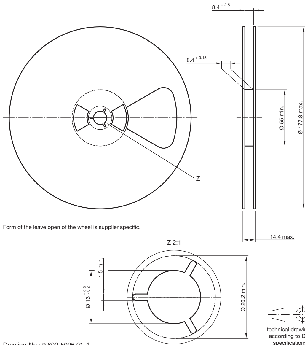
Fig. 11 - 7" Reel, 3000 Pieces
