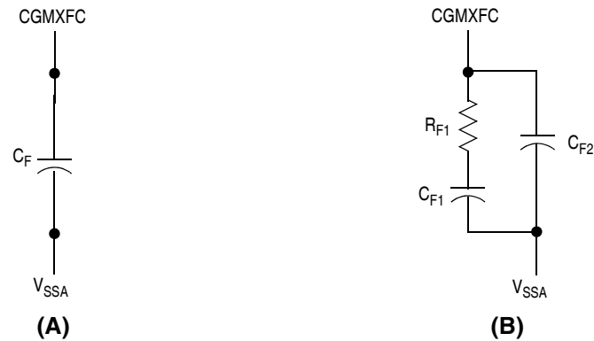
Figure 4-10. PLL Filter
