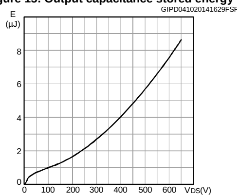
Figure 15: Output capacitance stored energy
