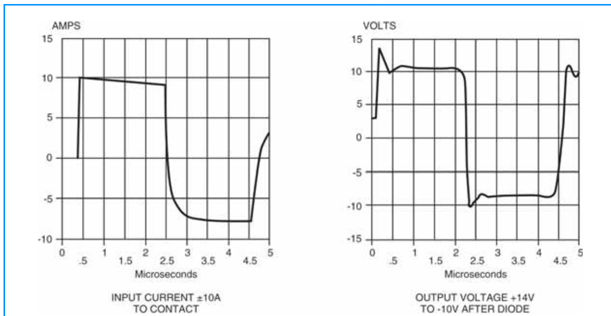
DIODE CONTACT PULSE TEST, ±5.8 DIODE
