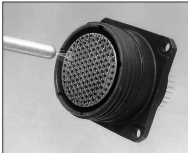
ESD Testing on MIL-DTL-38999, Series III Filter Cylindrical Connector (Actual Photo)
