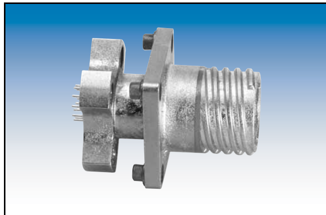
Composite FCTV Connector for PCB board mounting. Amphenol is currently the only supplier of one-piece composite PCB stand-off shells.
