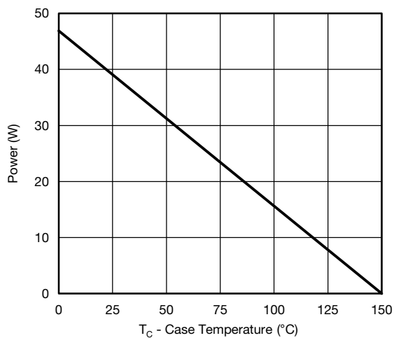
Power, Junction-to-Case
