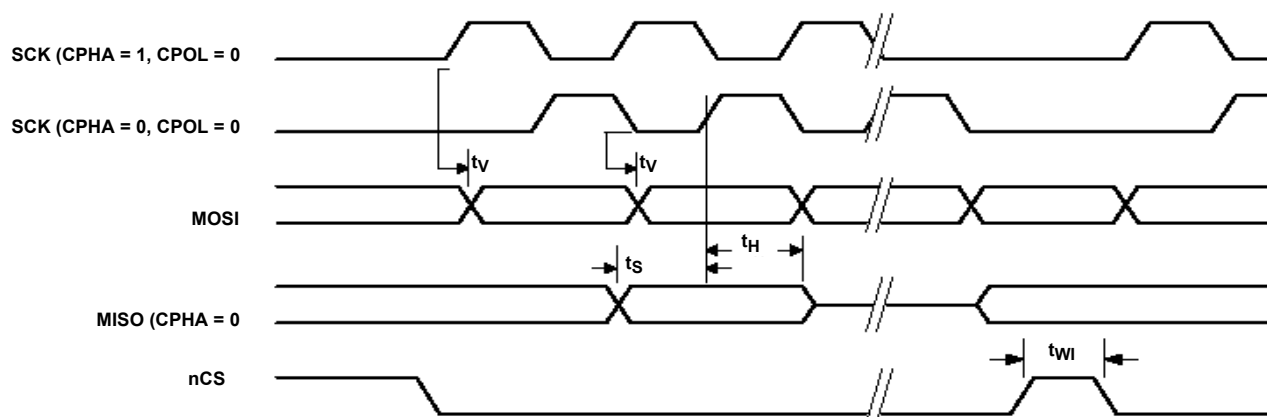
FIGURE 5. SPI TIMING
