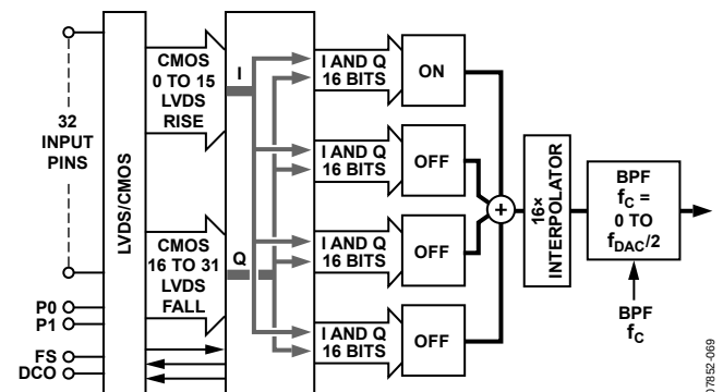
Figure 93. QDUC Mode
