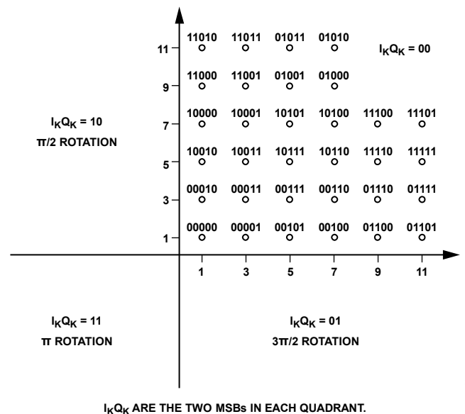
Figure 124. DVB-C 128-QAM Constellation3
