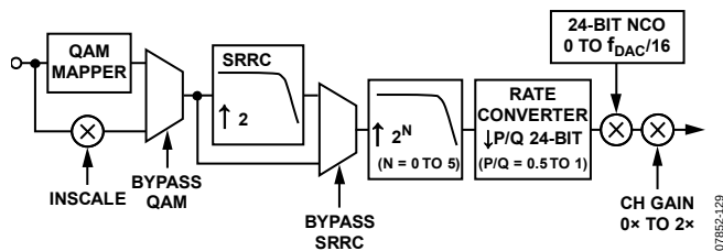
Figure 71. Datapath Block Diagram
