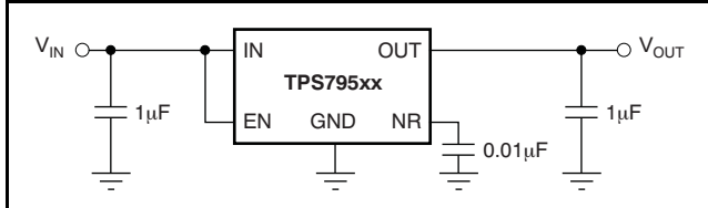
Figure 23. Typical Application Circuit
