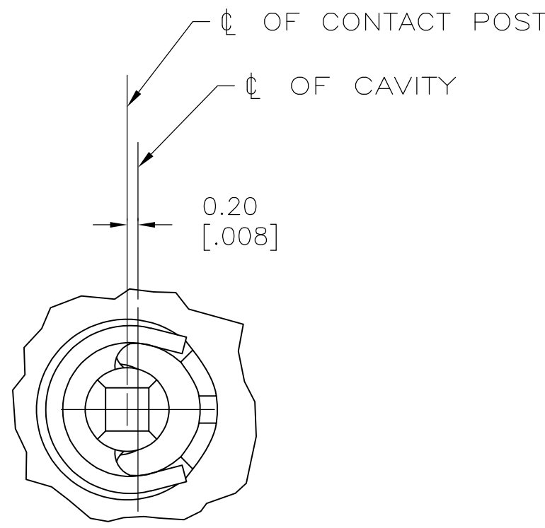
VIEW C-C SCALE 10:1 2 PLC 788194-6 ONLY
