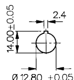
Fixing Details
