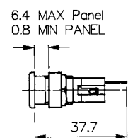
Fixing Details
