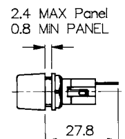
Fixing Details
