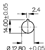
Fixing Details
