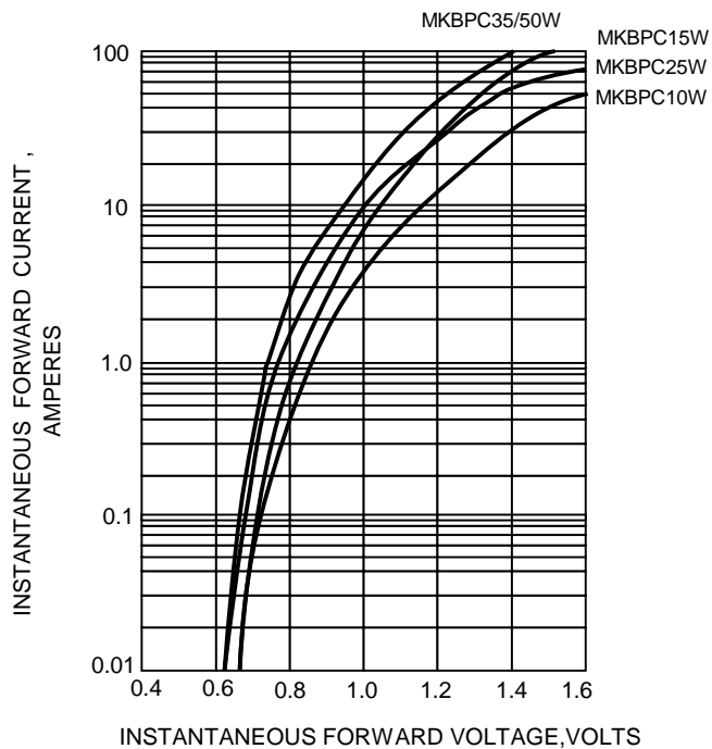
FIG.3-TYPICAL FORWARD CHARACTERISTICS
