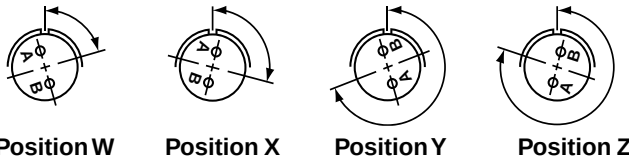
Position W Position X Position Y Position Z View looking into front face of pin insert or rear of socket insert.
