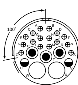
100° Rotation of 32-6
