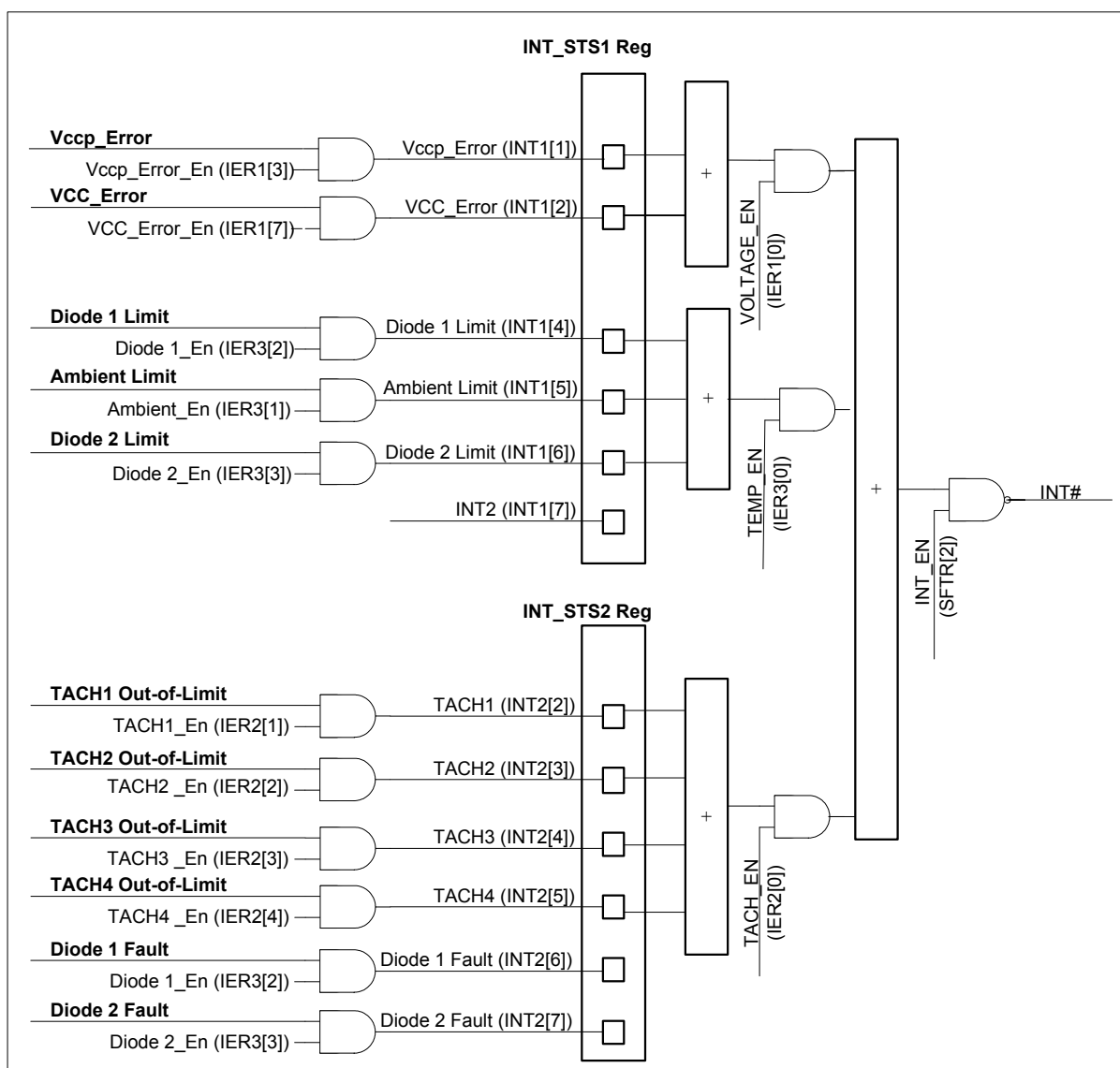
Figure 6.3 Interrupt Control
