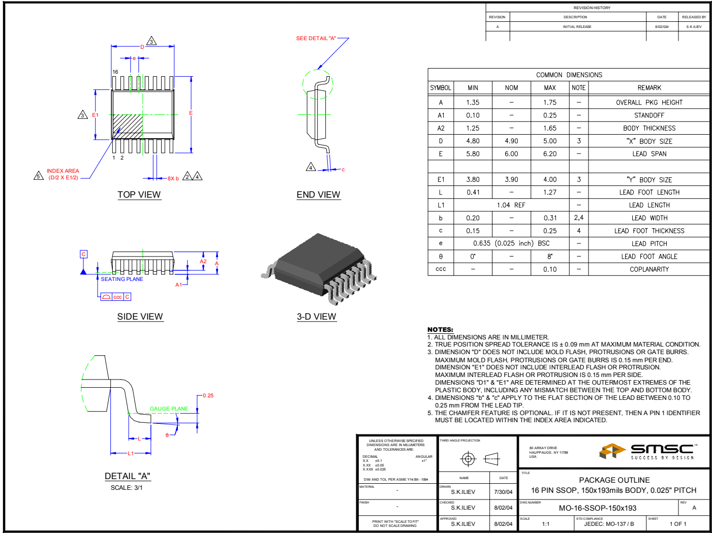
Figure 10.1 16 Pin SSOP Package Outline and Parameters
