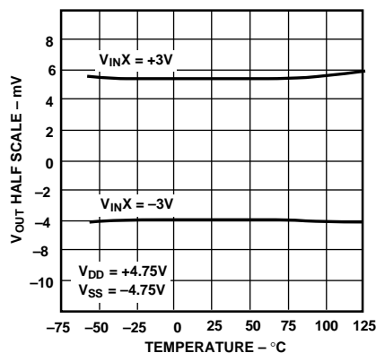
Figure 6. V_{OUT} Half Scale ( 80_H ) vs. Temperature
