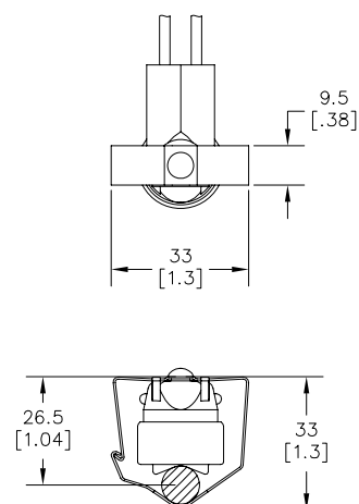
Locking Tube Mount Clip (3/8 Inch Shown)
