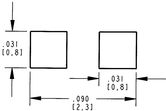
RECOMMENDED SOLDERING PAD LAYOUT
