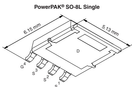
N-Channel MOSFET
