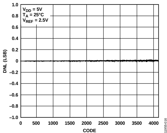
Figure 16. AD5681R DNL
