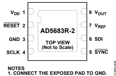
Figure 8. Pin Configuration, 8-Lead LFCSP, \overline{\text{RESET}} Option
