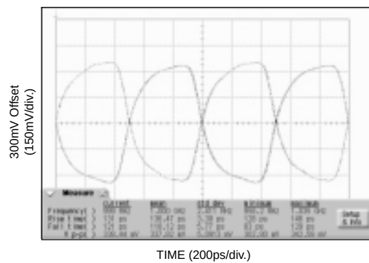
1GHz Output
