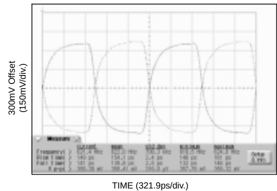
622MHz Output
