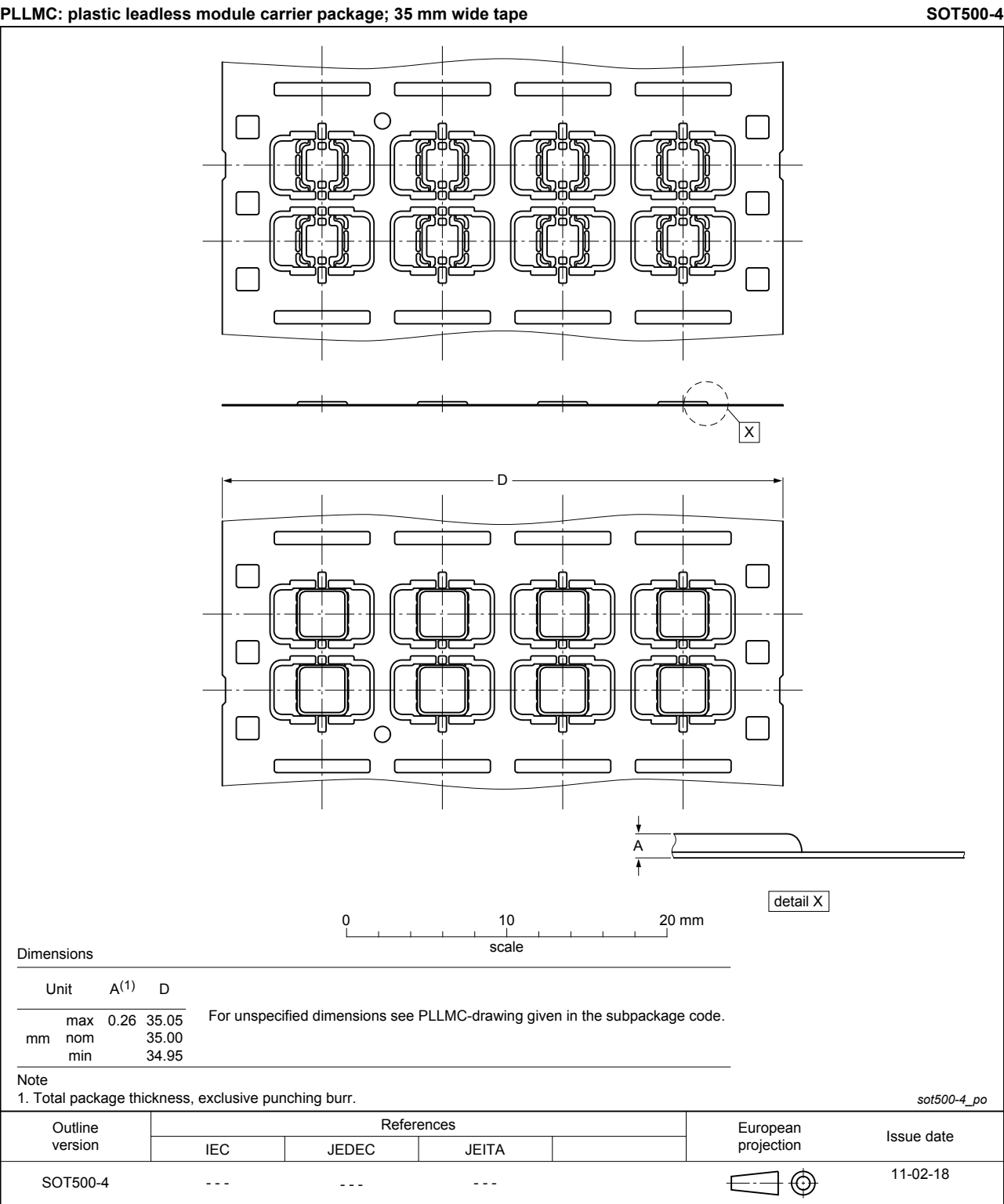
Figure 7. Package outline SOT500-4
