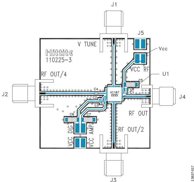
Figure 17. Evaluation PCB
