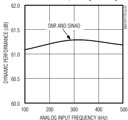
DYNAMIC PERFORMANCE vs. INPUT FREQUENCY (MAX1077)
