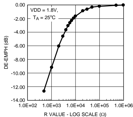
Figure 21. De-Emph vs. R value
