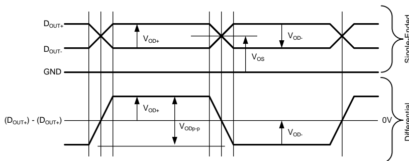
Figure 4. Serializer Output Waveforms
