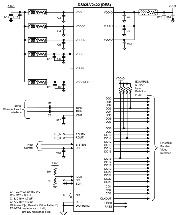
Figure 35. DS92LV2422 Typical Connection Diagram — Pin Control
