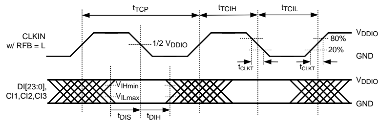
Figure 6. Serializer Input CLKIN Waveform and Set and Hold Times
