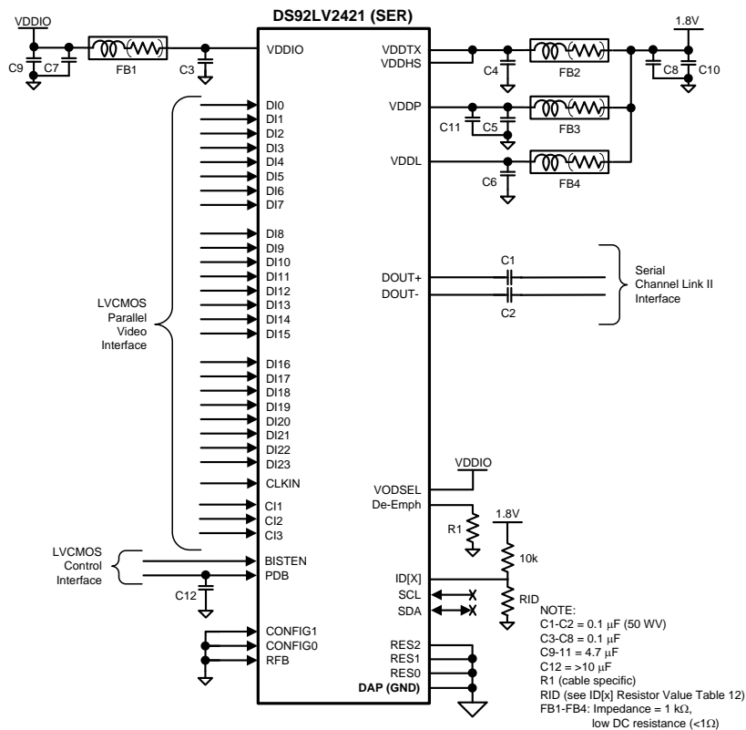
Figure 34. DS92LV2421 Typical Connection Diagram — Pin Control
