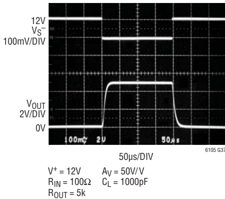
Step Response V_{SENSE} = 0\text{V to } 100\text{mV}, C_L = 1000\text{pF}, V_{S^+} = 12\text{V}
