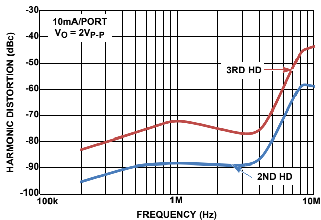
FIGURE 10. HARMONIC DISTORTION vs FREQUENCY
