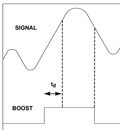
FIGURE 29. SERIAL TIMING DIAGRAM
