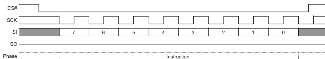
Figure 117. Mode Bit Reset Command Sequence
