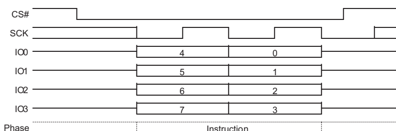
Figure 116. Software Reset Command Sequence QPI Mode
