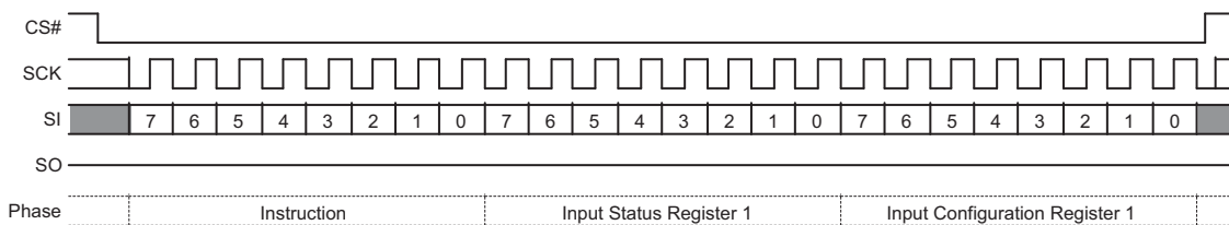
Figure 59. Write Registers (WRR) Command Sequence – 16-Data Bits
