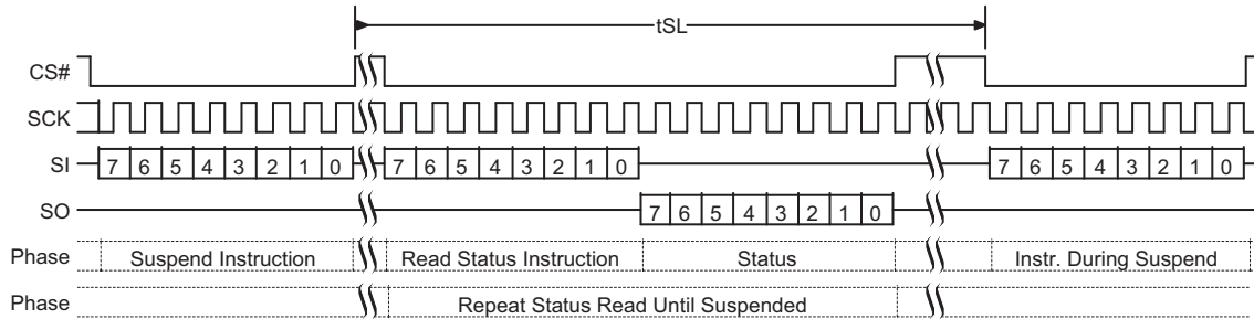
Figure 97. Program or Erase Suspend Command Sequence
